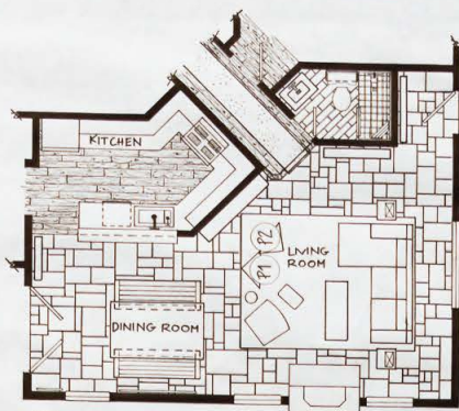
FLOOR PLAN SCALE: \frac{1}{4}" = 1'-0"
